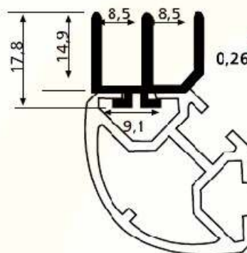
8 0.625 kg/m
