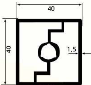
SK 701 0.950 kg/m
