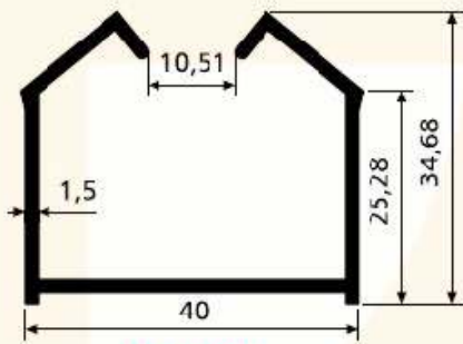
SM 1082/A 0.542 kg/m
