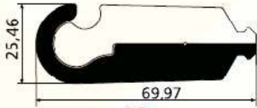
9/B 1,993 kg/m
