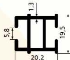
SM 1061/K 0.333 kg/m
