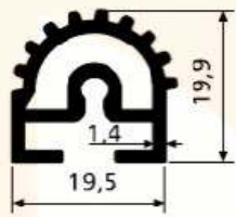
SM 1061/J 0.404 kg/m
