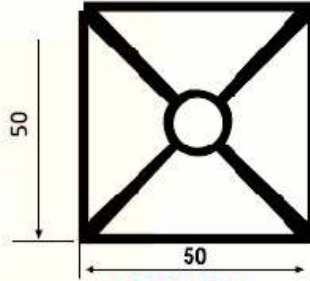
SK 5009 B 1.893 Kg/m
