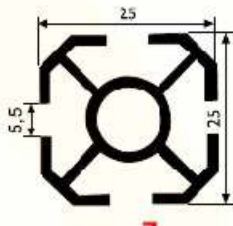
7 0.415 kg/m
