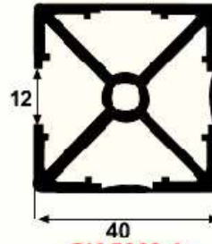
SK 5009 A 1.210 Kg/m
